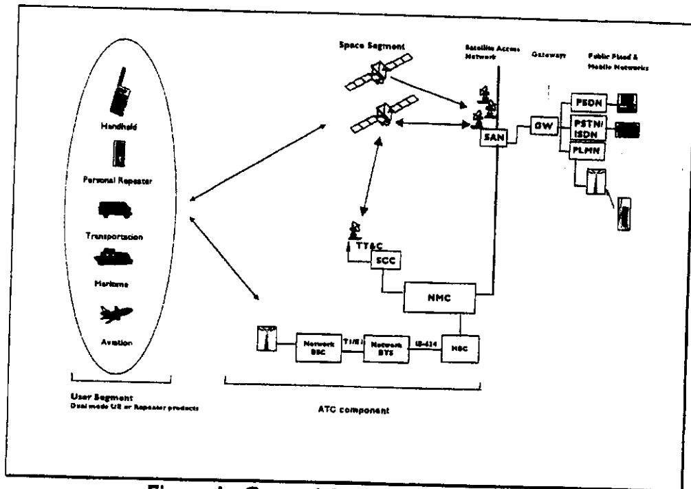
Figure 1: General Architecture of Integrated MSS Network with ATC
